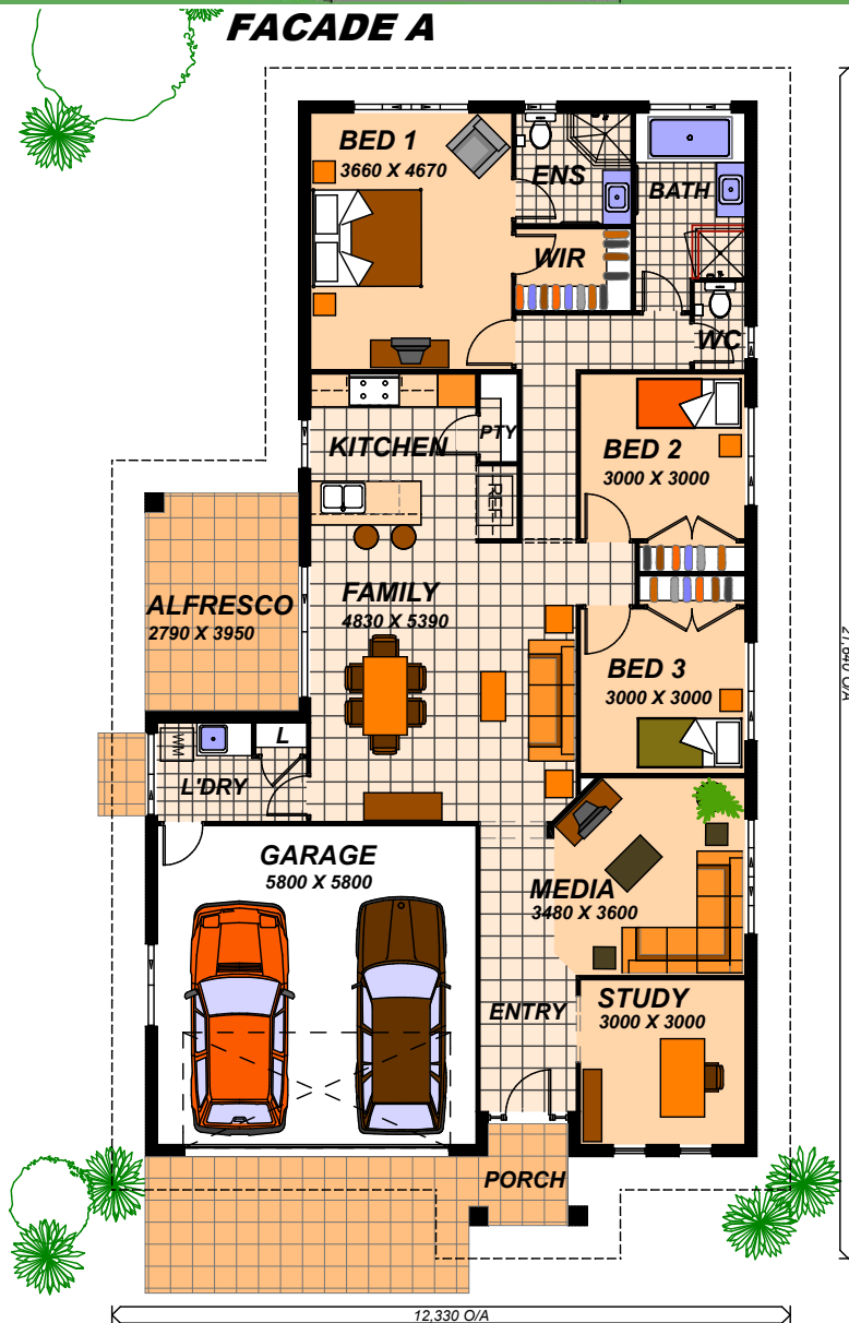
FLOOR PLAN
