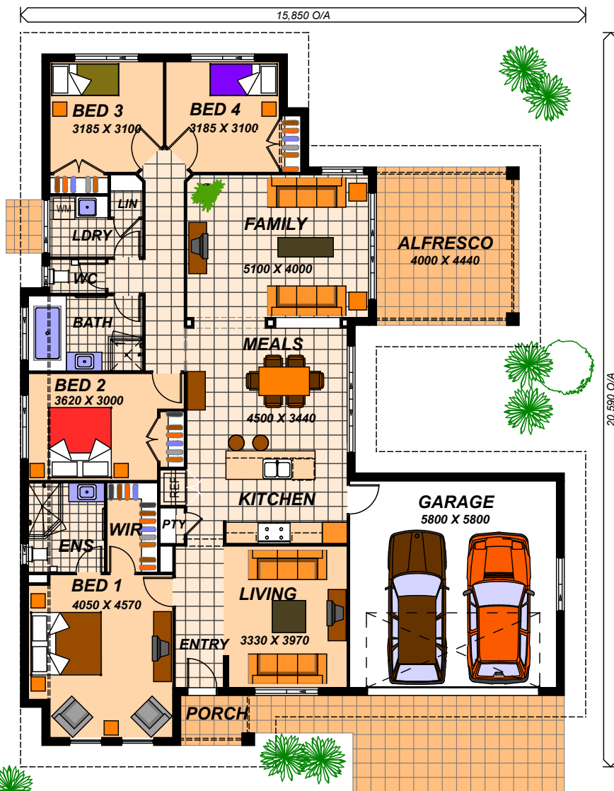
FLOOR PLAN
