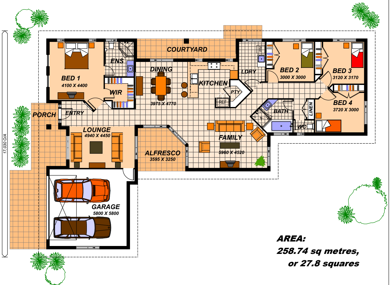
FLOOR PLAN
