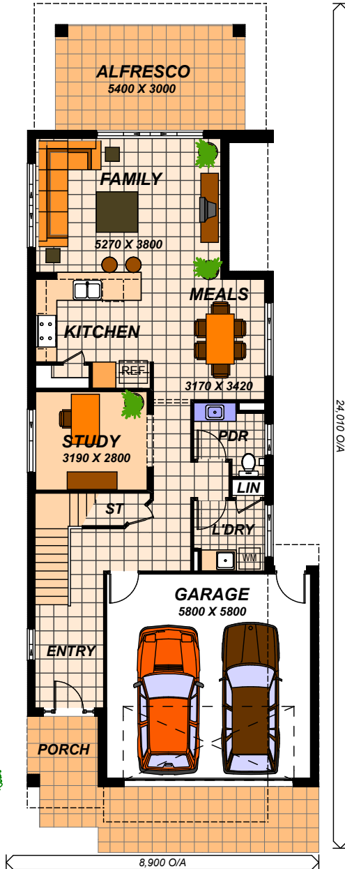
GROUND FLOOR
